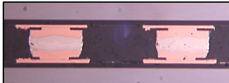
20 \mu\text{m} Copper Pillar SnAgCu Solder Cap
